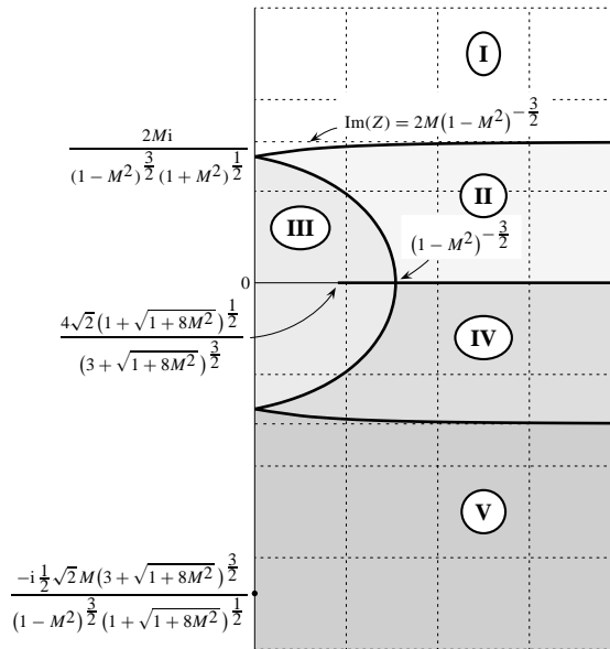
Figure 3.2 Complex impedance Z -plane, with regions of different numbers of surface waves. No solutions in I, \sigma_{HI} \in \text{II} \dots \text{V} , \sigma_{SR} \in \text{III} \dots \text{V} , \sigma_{SL} \in \text{IV} \dots \text{V} , \sigma_{HS} \in \text{V} . Thick lines map to the branch cuts in figure 3.3. In the figure M = 0.5 is taken.
