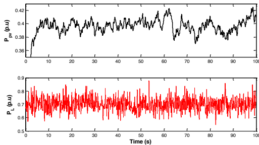
Fig. 3 Presents the output power of P_{PV} and load demand ( P_L )
