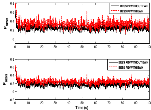
Fig. 4 Output power of BESS with and without EWH subject to PI and PID controllers
