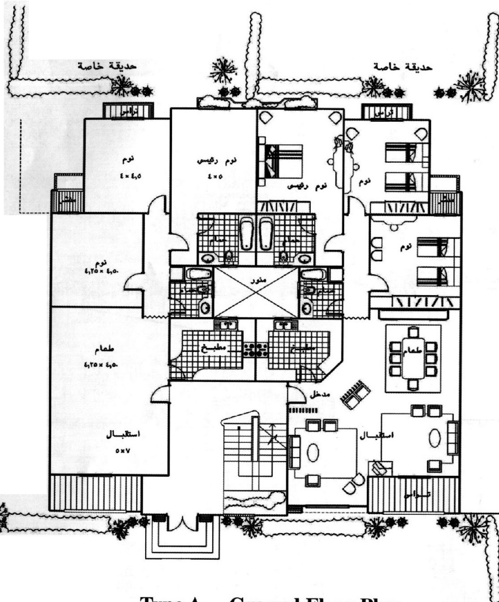
Type A--- Ground Floor Plan
