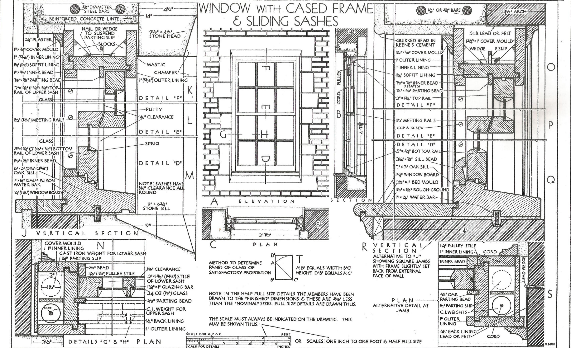
ALTERNATIVELY, THE SHEET MAY CONSIST OF 'A', 'B' & 'C' WITH DETAILS 'J' & 'N' ON THE LEFT & RIGHT RESPECTIVELY T Y P I C A L H O M E W O R K S H E E T 1/8" HIGH LETTERING FOR DESCRIPTION SHOULD BE BETWEEN GUIDE LINES FIGURE 60
