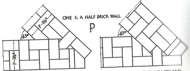
ALTERNATE COURSES SHOWING BIRDSMOUTHED ACUTE SQUINT QUOIN IN DOUBLE FLEMISH BOND
