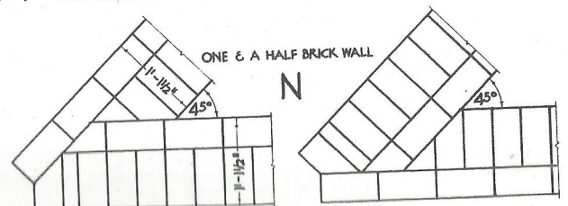
ALTERNATE COURSES SHOWING BIRDSMOUTHED ACUTE SQUINT QUOIN IN ENGLISH BOND
