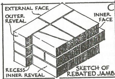
REBATED JAMBS WITH 2 1/4" RECESSES
