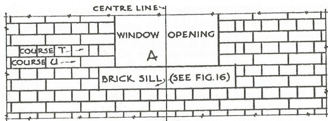
FRONT ELEVATION SHOWING 3" THICK BRICKS
