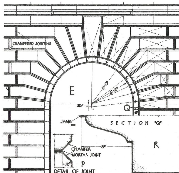
DETAIL OF JOINT
