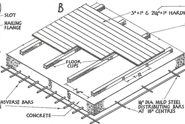
REINFORCED CONCRETE FLOOR WITH BEARERS & BOARDING
