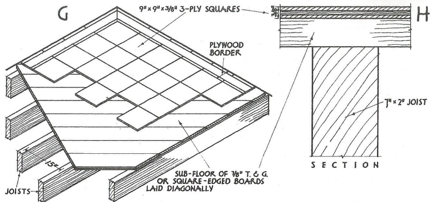
PLYWOOD FLOORING ON WOOD SUB-FLOOR
