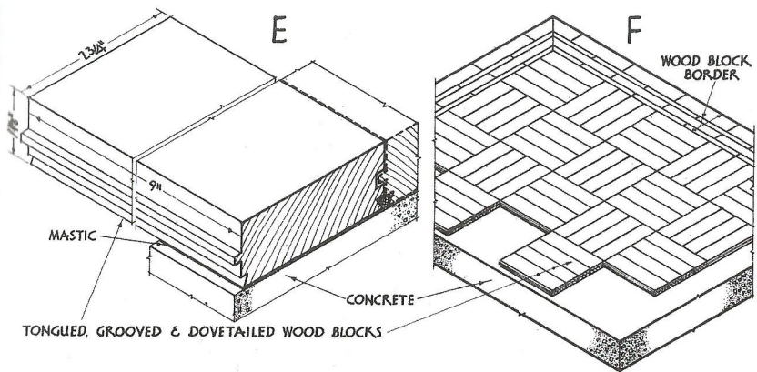
WOOD BLOCK FLOORING ON CONCRETE SUB-FLOOR
