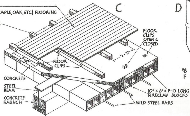
HOLLOW BLOCK FLOOR WITH BEARERS & BOARDING
