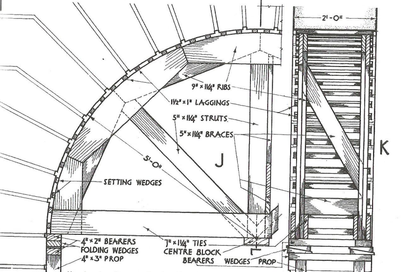
HALF ELEVATION CENTRE FOR STONE ARCH SIMILAR TO THAT SHOWN AT "A", FIGURE 37*
