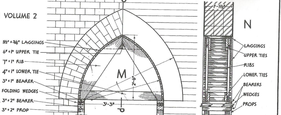
ELEVATION SECTION "PP" CENTRE FOR ARCH SHOWN AT "L", FIG. 19*
