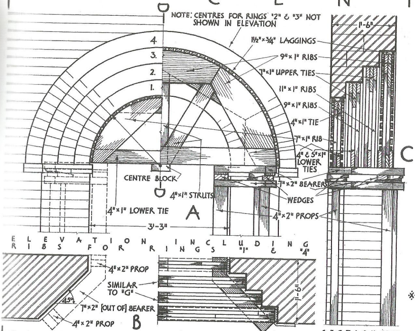
PLAN AT JAMB & ARCH CENTRE FOR STEPPED ARCH OF DOORWAY SHOWN AT "A", FIG. 19*
