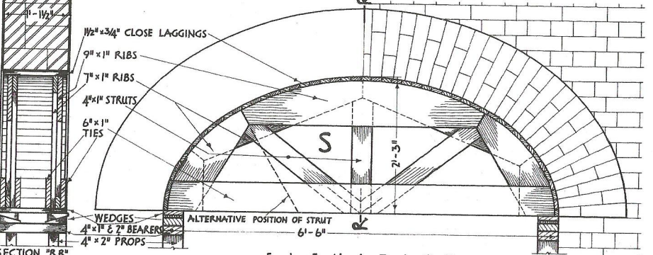
ELEVATION SECTION "RR" CENTRE FOR SEMI-ELLIPTICAL ARCH SHOWN AT "J", FIG. 19*
