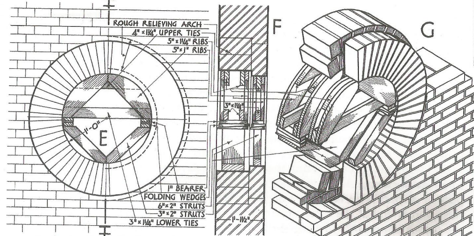
ELEVATION SECTION "HH" SKETCH CENTRE FOR CIRCULAR ARCH SHOWN AT "H", FIG. 19*
