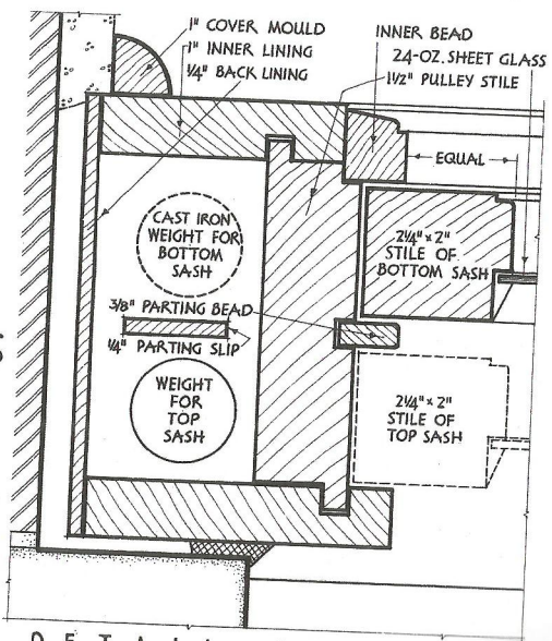
DETAIL AT JAMB
