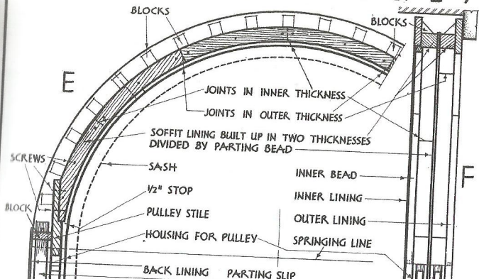
SECTION THROUGH HEAD OF FRAME
