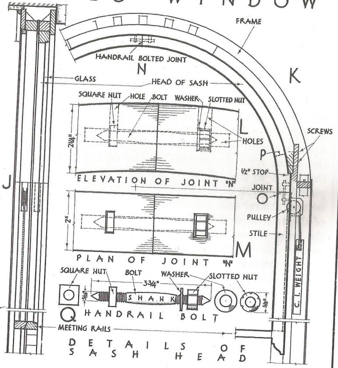
SECTION
