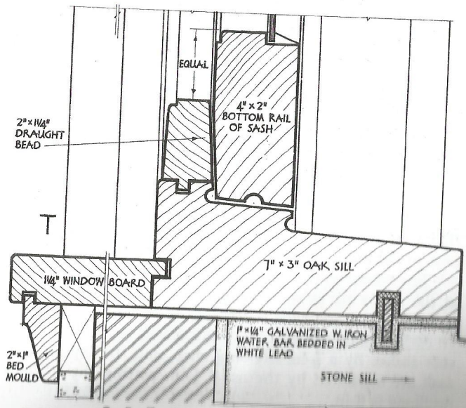
DETAIL AT SILL
