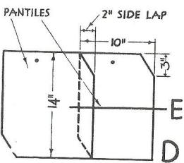
PLAN SHOWING SIDE LAP
