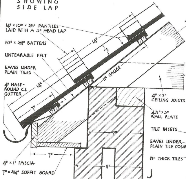
EAVES DETAIL
