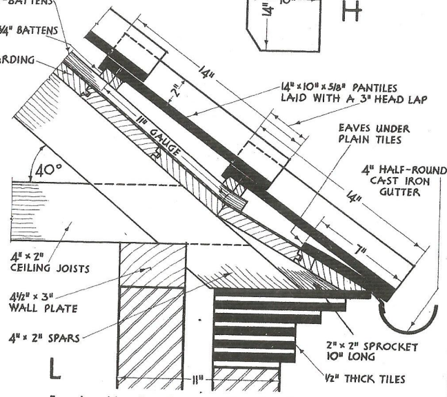
EAVES DETAIL
