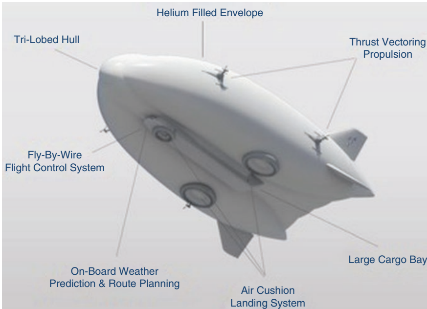
Fig. 21.14 Hybrid airship underside view highlighting the location and relative size of the cargo bay and air cushion landing system. (Image from Lockheed Martin, 2017,
