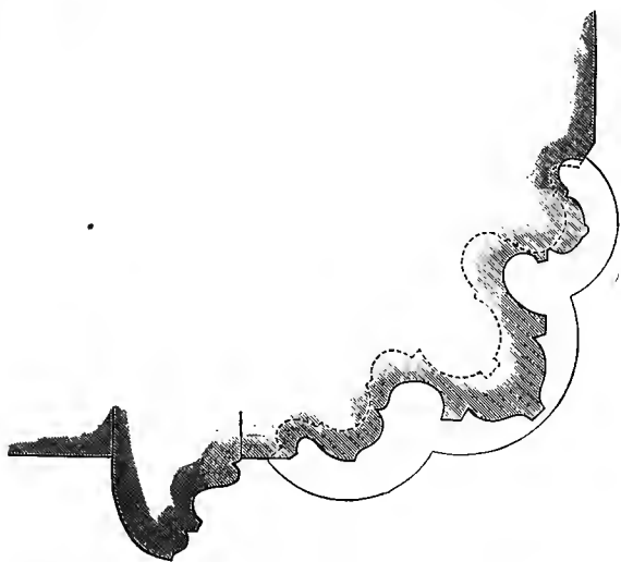
Priests' door, Heckington, Lincolnshire. Scale, 2 in. to 1 ft.
