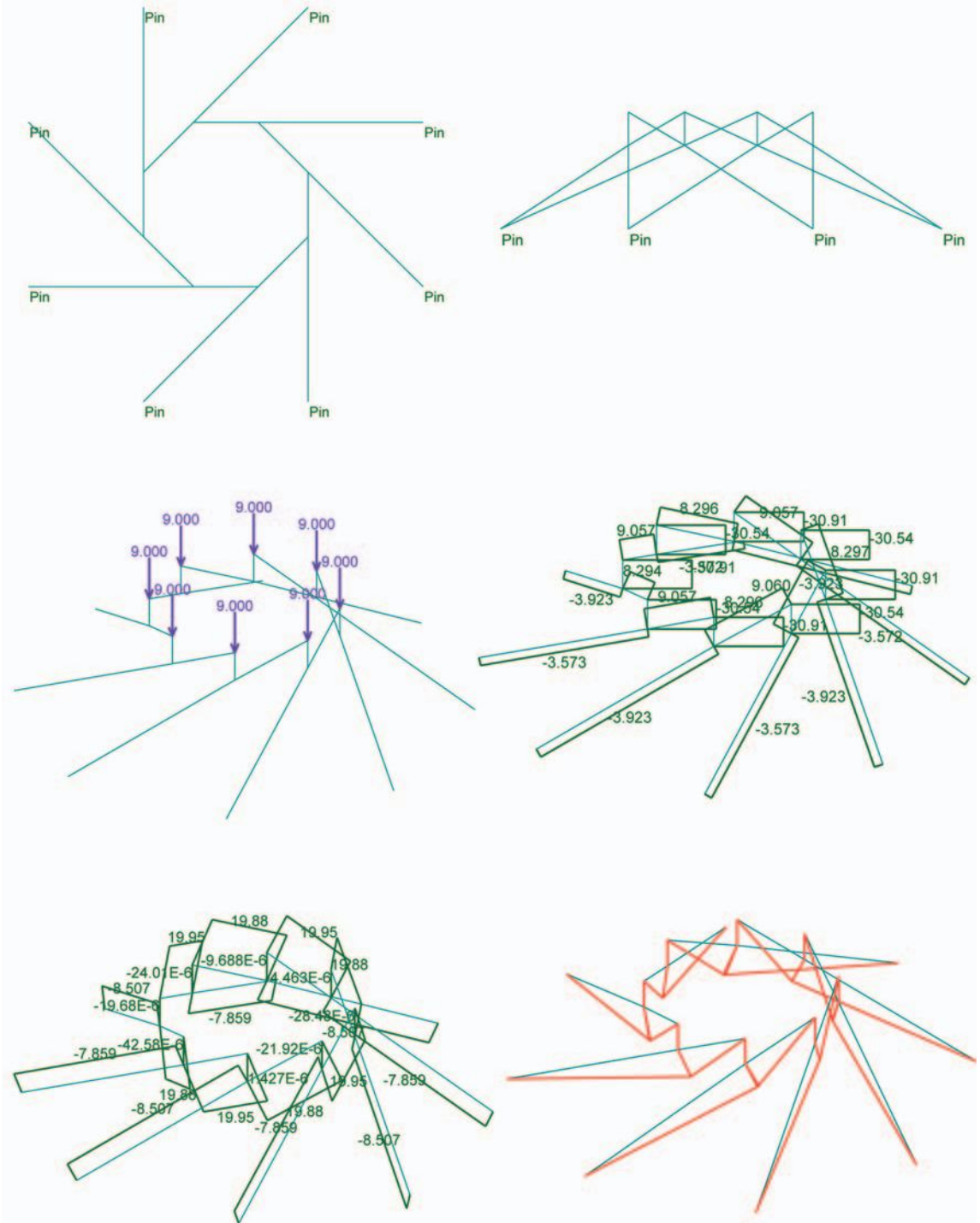
▲ 5.3 Model 3 – low-pitch RF structure with eight beams: plan, side elevation, loads, axial, shear and moment diagrams. (Drawings: Jens Larsen.)
