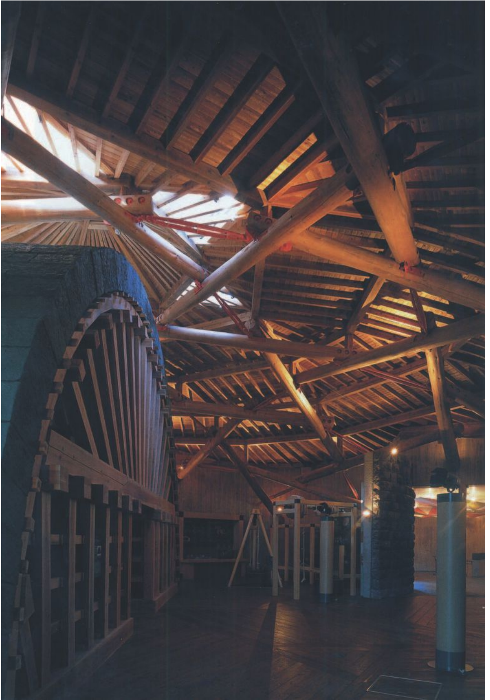
▲ 9.13 Interior view showing the permanent exhibit of a masonry bridge. (Photo: Keikaku-Inc.)
