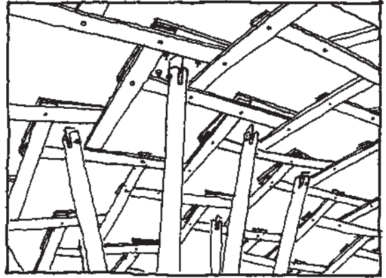
▲ 2.23 Rice University bamboo canopy by architect Sheguru Ban and engineer Cecil Balmond – detail. (Sketch by A. E. Piroozfar.)
