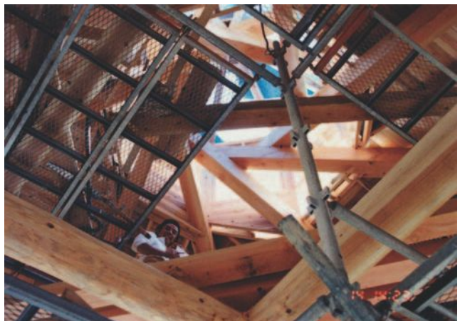
▲ 8.22 View through the roof light. (Photo: Yoichi Kan.)
