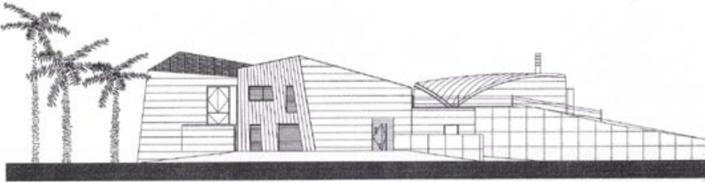
Alzado norte/North elevation
