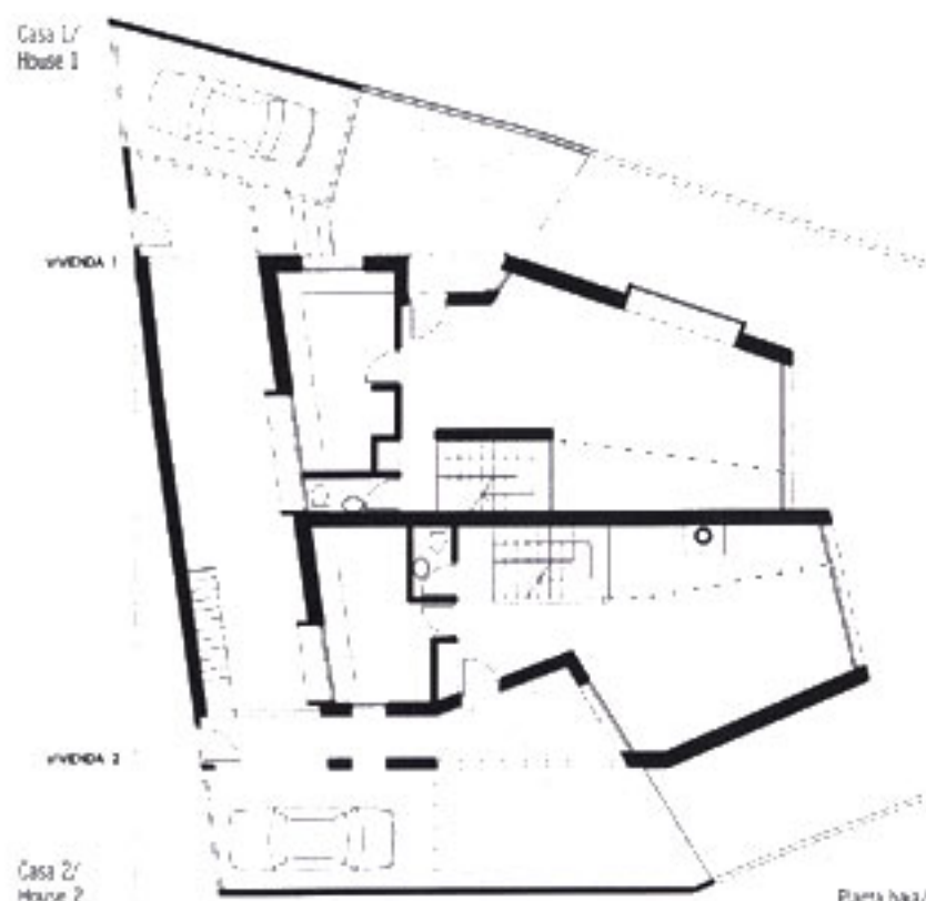
Panta baa/Ground floor
