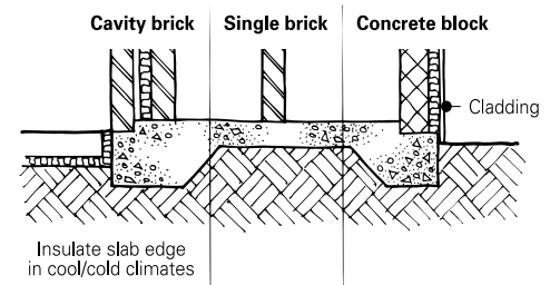
Examples of high mass construction
